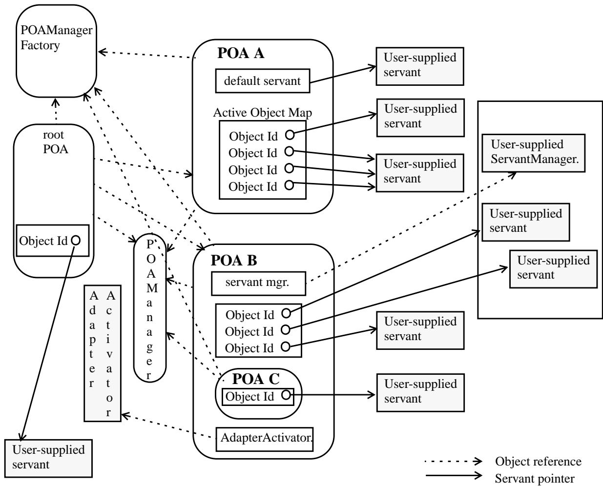
Figure 11-2 POA Architecture
