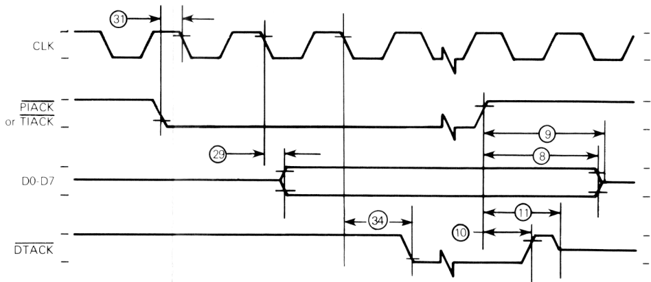
Figure 6-4. IACK Timing Diagram
