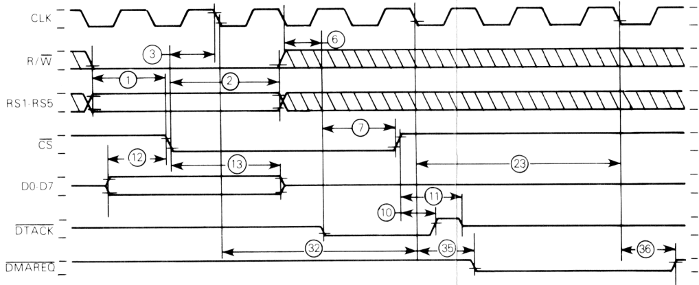
Figure 6-3. Write Cycle Timing Diagram
