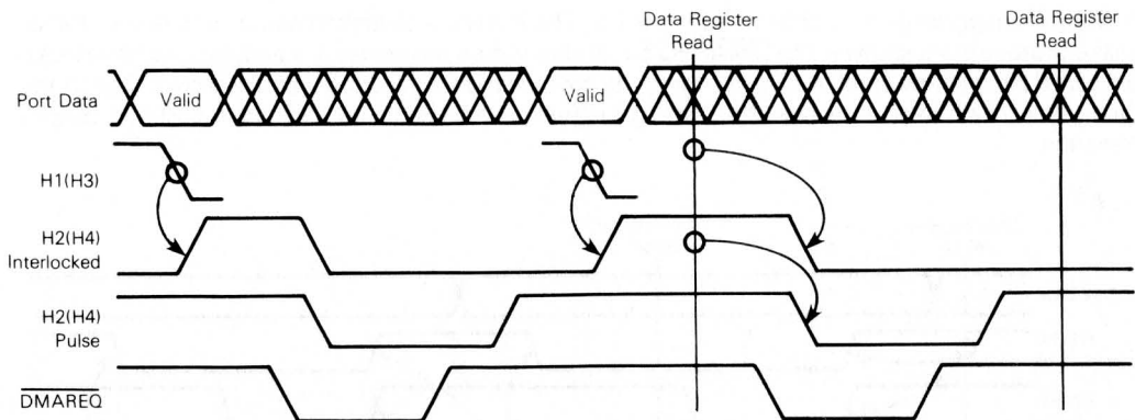
Figure 2-1. Double-Buffered Input Transfers Timing Diagram
