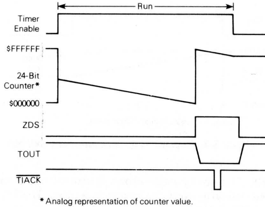
Figure 5-3. Single Interrupt After Timeout Example
