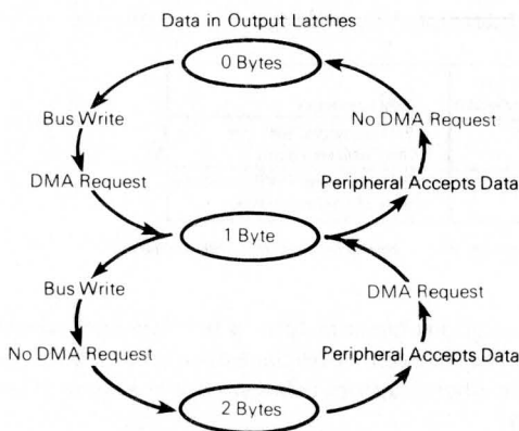
Figure 2-3. \overline{\text{DMAREQ}} Associated with Output Transfers
