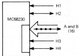
Figure 1-2. Port Mode Layout (Sheet 1 of 2)
