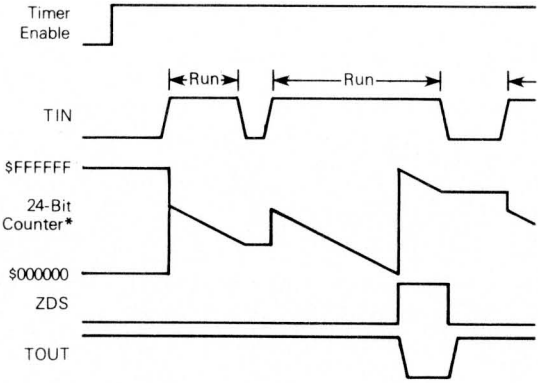
Figure 5-5. Device Watchdog Example
