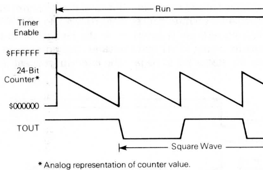
Figure 5-2. Square Wave Generator Example
