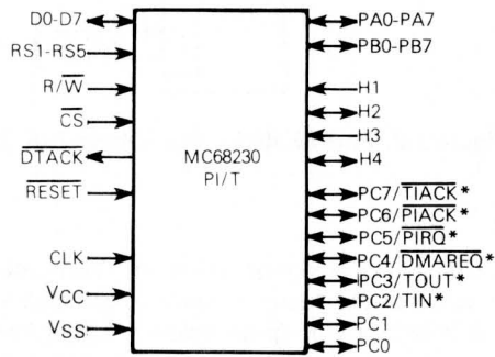
Figure 1-3. Logical Pin Assignment
