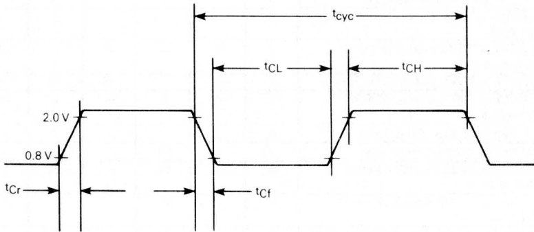
Figure 6-1. Clock Input Timing Diagram
