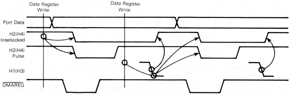
Figure 2-2. Double-Buffered Output Transfers Timing Diagram
