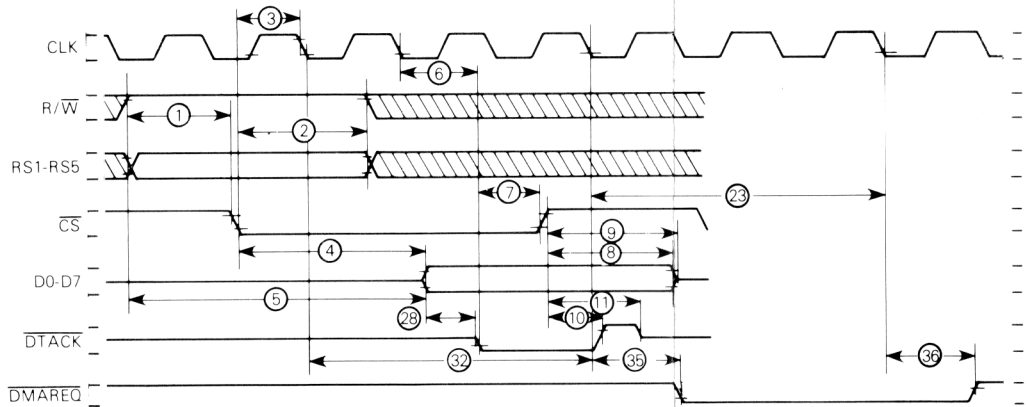
Figure 6-2. Read Cycle Timing Diagram
