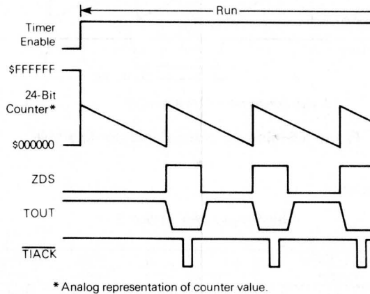
Figure 5-1. Periodic Interrupt Generator Example
