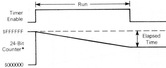
Figure 5-4. Elapsed Time Measurement Example
