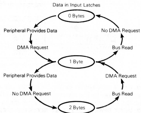
Figure 2-4. \overline{\text{DMAREQ}} Associated with Input Transfers
